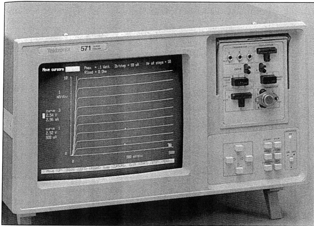
571 Curve Tracer
